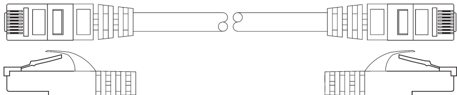
KOMMDATA PATCH CORD CAT.6A U/UTP 4PR 24AWG VERIFIED TO ISO/IEC 11801-1 CATEGORY 6A LSZH IEC 60332-1
